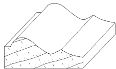
IH-204 1/2 x 1-1/4 cabinet moulding
