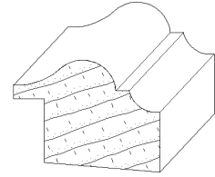
IH-1234 1-1/16 x 1-3/8 cabinet moulding
