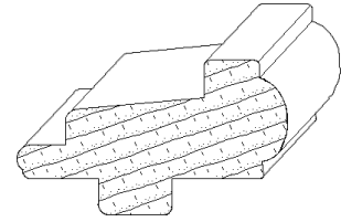
IH-1237 1-1/2 x 2-5/8 cabinet moulding
