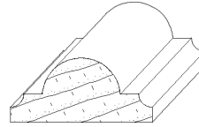
IH-278 9/16 x 1-3/8 cabinet moulding
