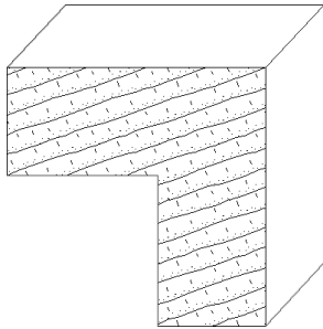
IH-274 2-1/4 x 2-1/4 cabinet moulding
