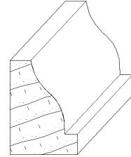
IH-1215 5/8 x 7/8 cabinet moulding
