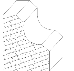
IH-1227 1-3/4 x 2-1/16 cabinet moulding
