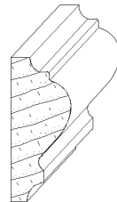
IH-1230 5/8 x 1-1/2 cabinet moulding
