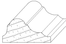
IH-237 3/4 x 1-1/2 cabinet moulding
