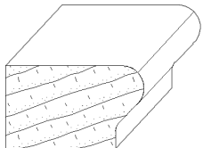
IH-1223 3/4 x 1-1/4 cabinet moulding
