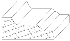
IH-211 3/4 x 1-3/4 cabinet moulding
