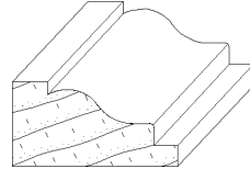
IH-295 9/16 x 1-1/8 cabinet moulding
