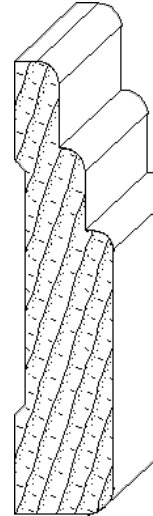
IH-1412 7/8 x 4 casing moulding
