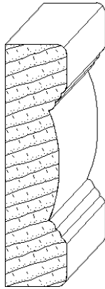
IH-14010 13/16 x 3-3/16 casing moulding
