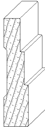
IH-1485 3/4 x 3-1/4 casing moulding
