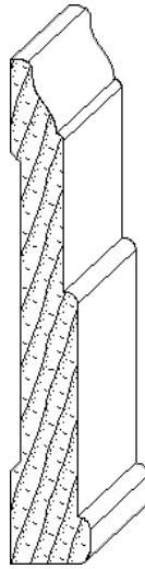
IH-434 3/4 x 4-5/8 casing moulding
