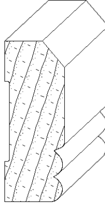
IH-423 3/4 x 2 casing moulding
