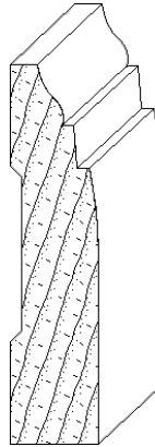
IH-1470 3/4 x 3-1/2 casing moulding
