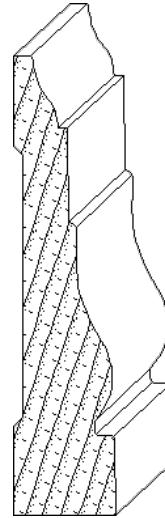
IH-467 1 x 4-1/2 casing moulding
