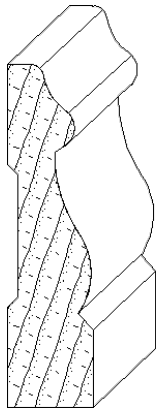
IH-471 3/4 x 3 casing moulding
