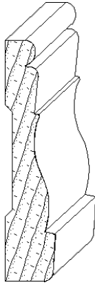
IH-4002 (MC131) 11/16 x 3-1/4 casing moulding
