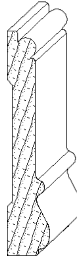
IH-1443 3/4 x 4 casing moulding
