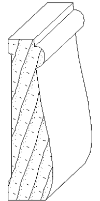
IH-455 5/8 x 2-1/4 casing moulding
