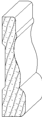
IH-1472 3/4 x 3-1/4 casing moulding
