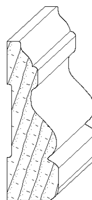
IH-416 3/4 x 2-5/16 casing moulding
