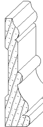
IH-1489 3/4 x 3-1/4 casing moulding
