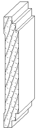
IH-436 1/2 x 3-3/4 casing moulding
