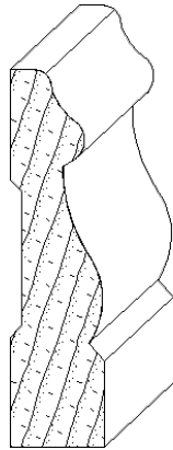
IH-1446 3/4 x 3 casing moulding
