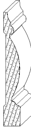
IH-1469 3/4 x 5 casing moulding
