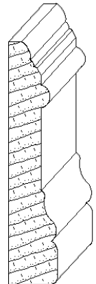
IH-14005 11/16 x 3-1/2 casing moulding
