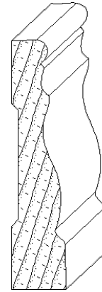
IH-459 3/4 x 3-7/16 casing moulding
