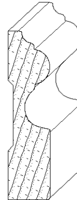
IH-463 3/4 x 3 casing moulding
