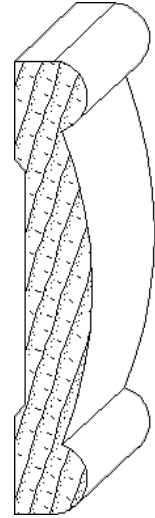
IH-1456 11/16 x 4 casing moulding
