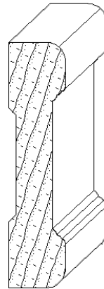
IH-494 3/4 x 3-1/4 casing moulding
