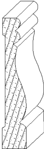
IH-481 3/4 x 4 casing moulding
