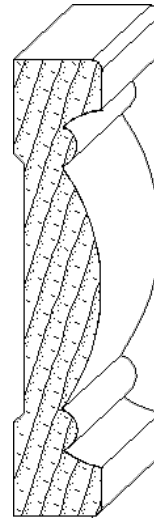
IH-1475 13/16 x 4-1/4 casing moulding
