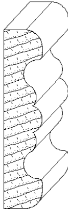
IH-14008 3/4 x 3-1/2 casing moulding
