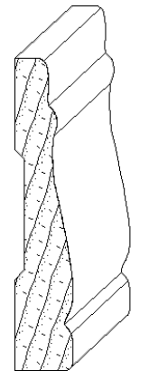
IH-1426 9/16 x 3 casing moulding
