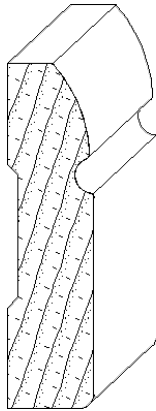
IH-1444 3/4 x 3 casing moulding
