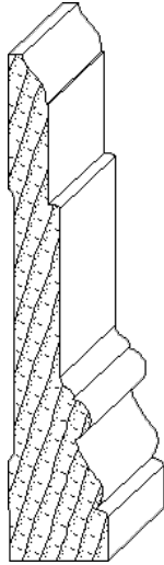
IH-442 1 x 5 casing moulding
