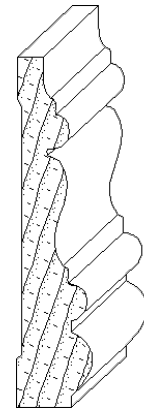
IH-465 3/4 x 3-1/2 casing moulding
