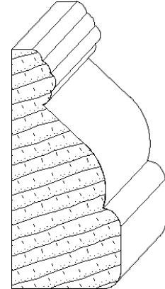
IH-14003 1-1/4 x 2-3/4 casing moulding
