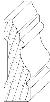
IH-1477 3/4 x 2-1/4 casing moulding
