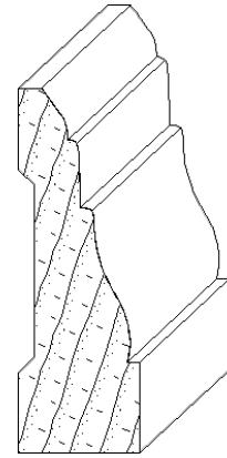
IH-1432 3/4 x 2-1/4 casing moulding
