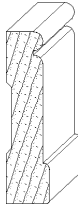
IH-1435 3/4 x 3 casing moulding
