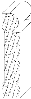
IH-448 3/4 x 3-1/2 casing moulding
