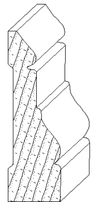
IH-466 1 x 3-1/4 casing moulding
