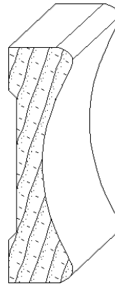
IH-433 3/4 x 2-3/4 casing moulding
