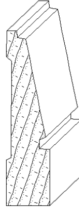
IH-409 11/16 x 3 casing moulding
