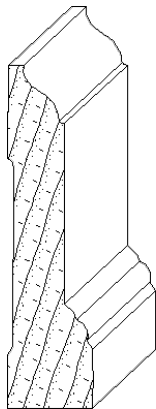
IH-435 3/4 x 3 casing moulding
