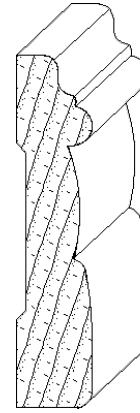
IH-1437 3/4 x 3 casing moulding
