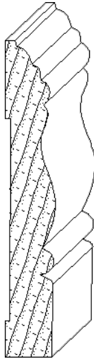
IH-472 11/16 x 4-5/16 casing moulding
