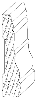
IH-417 3/4 x 3-1/4 casing moulding
