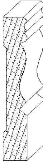
IH-1449 3/4 x 4-1/2 casing moulding
