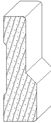
IH-1460 1-1/8 x 3-1/2 casing moulding
