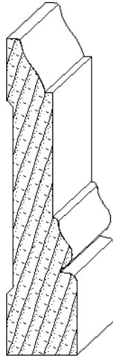
IH-447 1 x 4-1/2 casing moulding
