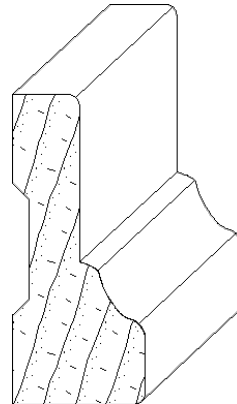
IH-1411 3/4 x 1-3/4 casing moulding
