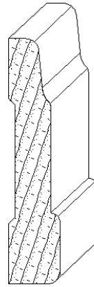
IH-495 3/4 x 3-9/16 casing moulding
