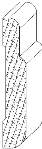
IH-1407 3/4 x 4-3/16 casing moulding
