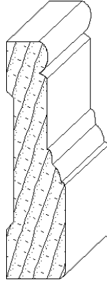
IH-407 3/4 x 3 casing moulding
