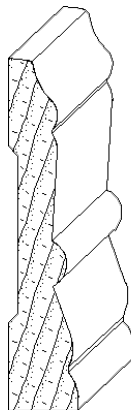
IH-1402 11/16 x 3-1/2 casing moulding
