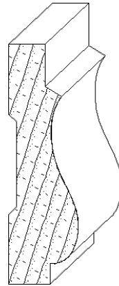
IH-1453 7/8 x 3 casing moulding
