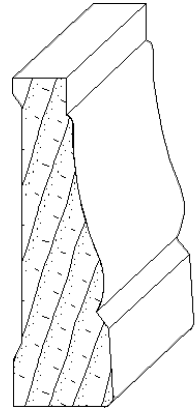
IH-444 11/16 x 2-1/4 casing moulding
