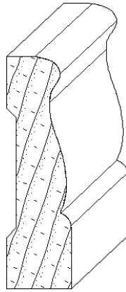
IH-1418 5/8 x 2-1/4 casing moulding
