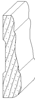
IH-478 11/16 x 3 casing moulding
