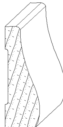
IH-452 3/4 x 2-3/16 casing moulding
