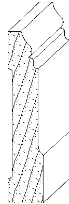
IH-1455 5/8 x 3 casing moulding
