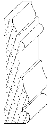
IH-430 3/4 x 3 casing moulding
