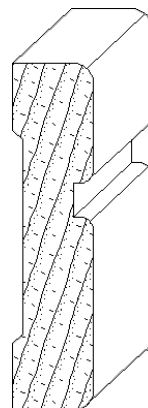
IH-1520-M 3/4 x 3-1/4 casing moulding
