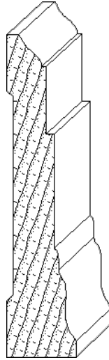
IH-449 1-1/16 x 5 casing moulding
