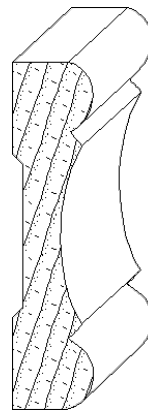
IH-428 3/4 x 3-1/4 casing moulding
