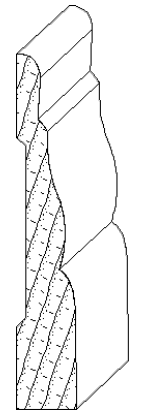
IH-1448 5/8 x 3-3/4 casing moulding
