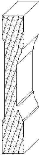
IH-480 3/4 x 4-3/4 casing moulding
