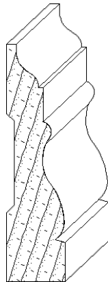
IH-1487 3/4 x 3 casing moulding
