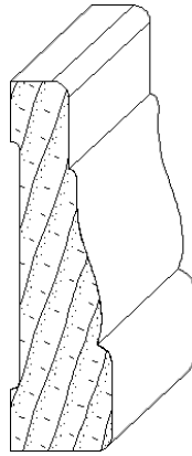
IH-461 11/16 x 2-1/2 casing moulding
