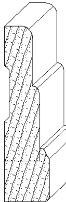
IH-1409 1 x 3-7/8 casing moulding
