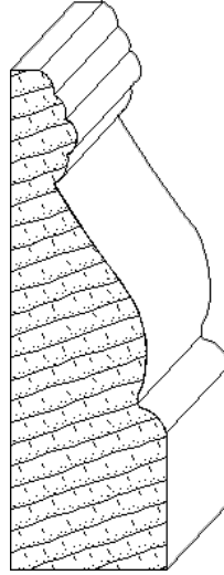
IH-1496 1-1/4 x 4 casing moulding
