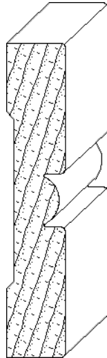
IH-1403 3/4 x 4 casing moulding
