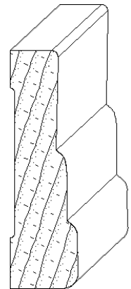
IH-451 3/4 x 2-5/8 casing moulding
