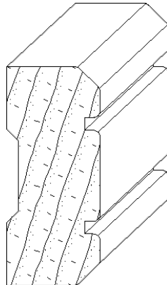
IH-1406 3/4 x 1-3/4 casing moulding
