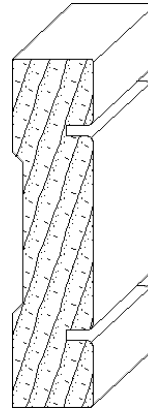
IH-1441 3/4 x 3-1/4 casing moulding
