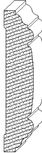
IH-485 1-9/16 x 7-3/8 casing moulding
