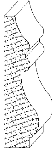
IH-14004 1-1/4 x 4-11/16 casing moulding
