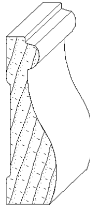
IH-1461 3/4 x 2-1/2 casing moulding
