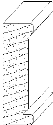
IH-14001 3/4 x 2-1/2 casing moulding
