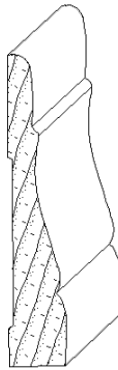
IH-404 3/4 x 3-5/16 casing moulding
