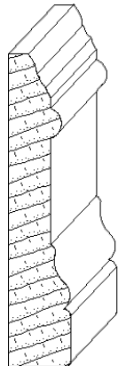
IH-4007 11/16 x 3-1/2 casing moulding
