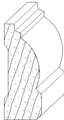
IH-1479 7/8 x 2-1/2 casing moulding
