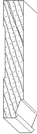
IH-1499 11/16 x 4 casing moulding
