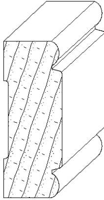
IH-405 3/4 x 2 casing moulding
