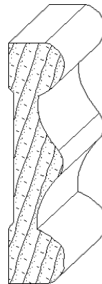
IH-458 3/4 x 3-1/4 casing moulding
