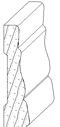
IH-498 1/2 x 2-1/4 casing moulding
