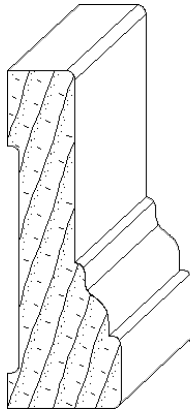
IH-468 7/8 x 2-5/8 casing moulding
