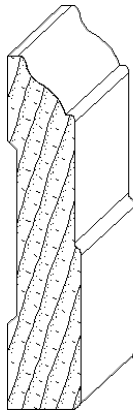
IH-489 3/4 x 3-5/8 casing moulding
