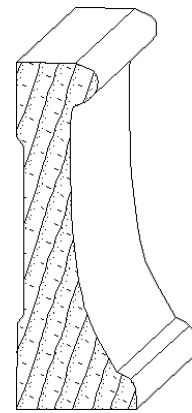
IH-431 1-1/16 x 3-1/4 casing moulding
