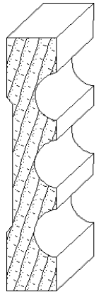
IH-486 3/4 x 3-1/4 casing moulding
