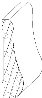
IH-453 5/8 x 2-3/16 casing moulding
