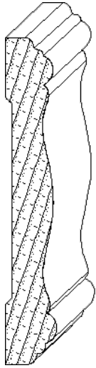
IH-403 3/4 x 4-3/4 casing moulding
