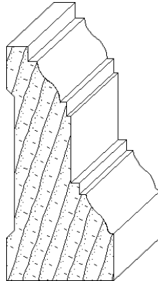
IH-1431 1-1/4 x 2-3/4 casing moulding
