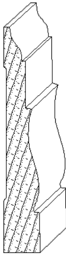
IH-408 3/4 x 4-9/16 casing moulding
