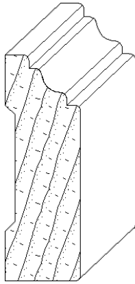
IH-1416 3/4 x 2-1/4 casing moulding
