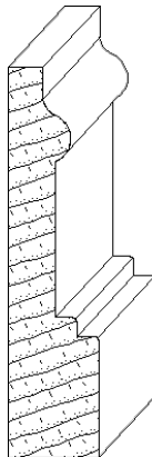
IH-4000 13/16 x 3-1/2 casing moulding
