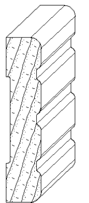
IH-414 9/16 x 2-5/8 casing moulding
