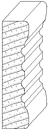
IH-1486 3/4 x 3 casing moulding
