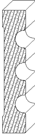
IH-482 1-1/4 x 6-1/2 casing moulding
