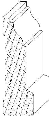
IH-1492 1 x 3-1/4 casing moulding
