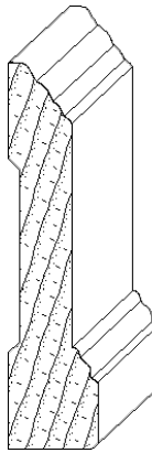
IH-410 13/16 x 3-1/2 casing moulding
