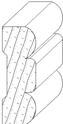
IH-1415 11/16 x 2 casing moulding
