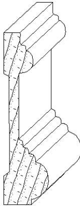
IH-413 3/4 x 2-7/8 casing moulding
