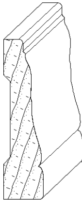
IH-1438 9/16 x 2-1/4 casing moulding
