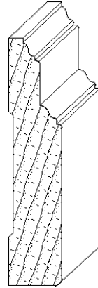
IH-1478 3/4 x 3-1/2 casing moulding
