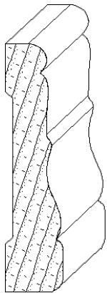
IH-479 3/4 x 3-1/4 casing moulding
