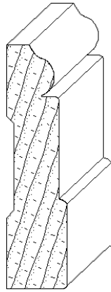
IH-1430 3/4 x 3 casing moulding
