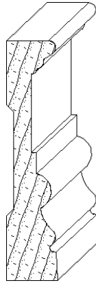
IH-1433 5/8 x 3-1/4 casing moulding
