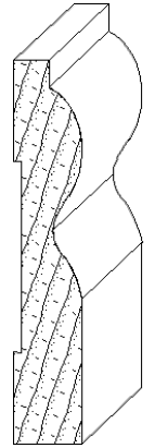
IH-456 5/8 x 3-1/2 casing moulding
