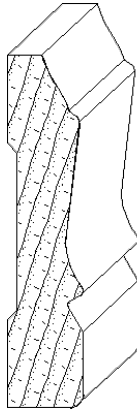
IH-1445 3/4 x 3-1/2 casing moulding
