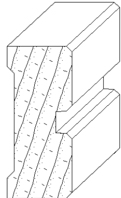
IH-1476 3/4 x 1-3/4 casing moulding
