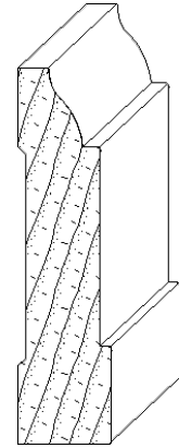
IH-1401 3/4 x 3 casing moulding
