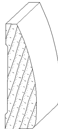
IH-426 3/4 x 2-1/2 casing moulding
