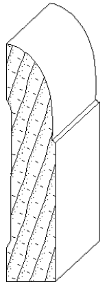
IH-445 5/8 x 3 casing moulding
