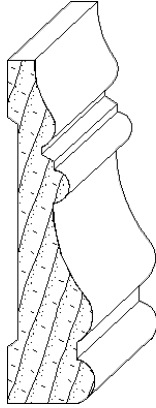
IH-406 3/4 x 3 casing moulding
