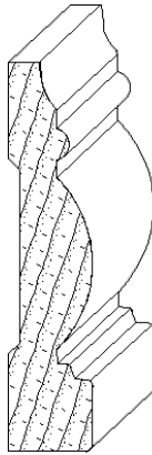
IH-1467 3/4 x 3-1/2 casing moulding
