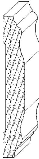
IH-427 3/4 x 4-7/8 casing moulding
