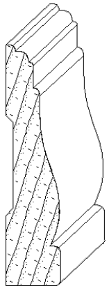
IH-1405 11/16 x 3 casing moulding
