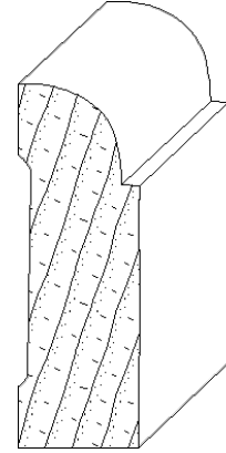
IH-425 3/4 x 2-1/4 casing moulding
