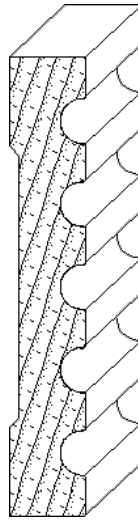
IH-1419 3/4 x 4-1/2 casing moulding
