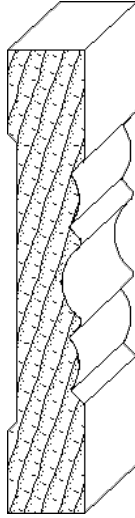
IH-1483 13/16 x 4-7/8 casing moulding
