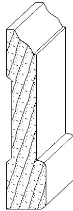
IH-1410 3/4 x 3-3/8 casing moulding
