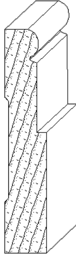
IH-429 3/4 x 4 casing moulding
