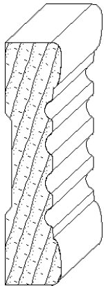
IH-438 3/4 x 3-1/4 casing moulding
