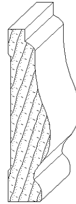
IH-457 13/16 x 3-5/8 casing moulding
