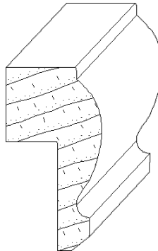
IH-320 13/16 x 1-9/16 chairrail_moulding
