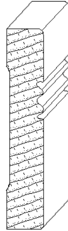
IH-330 3/4 x 4 chairrail_moulding
