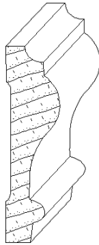
IH-305 5/8 x 2-1/2 chairrail_moulding
