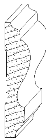
IH-323 3/4 x 3-3/8 chairrail_moulding
