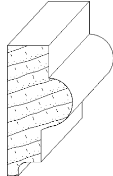
IH-375 13/16 x 1-5/8 chairrail_moulding
