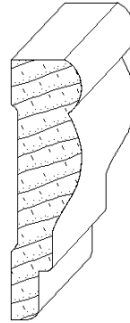
IH-332 11/16 x 2-1/2 chairrail_moulding
