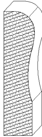
IH-759 1-5/8 x 6-5/8 rails_moulding
