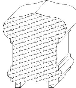
IH-729 2-3/4 x 3-1/4 rails_moulding
