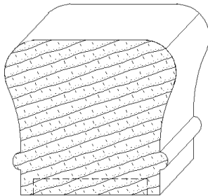
IH-732 2-3/8 x 2-5/8 rails_moulding
