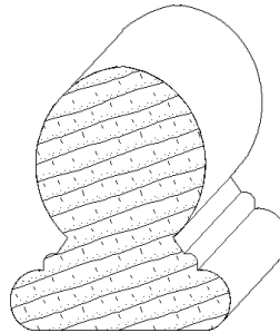
IH-705 2 x 2-3/8 rails_moulding
