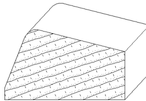
IH-738 1-1/2 x 2-1/2 rails_moulding
