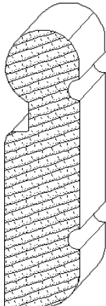
IH-709 1-1/2 x 5-1/2 rails_moulding
